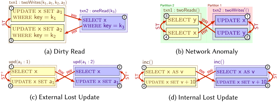
Fig. 14. Examples of dependency cycles generated by CLOTHO
