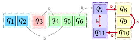
Fig. 13. An anomaly constructed by CLOTHO
