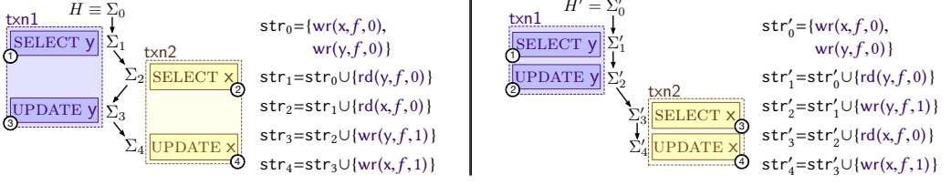
Fig. 10. A serializable execution (left) and its equivalent serial execution (right)
