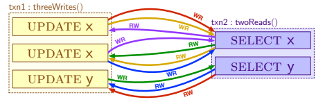
Fig. 19. Structurally Similar Anomalies
